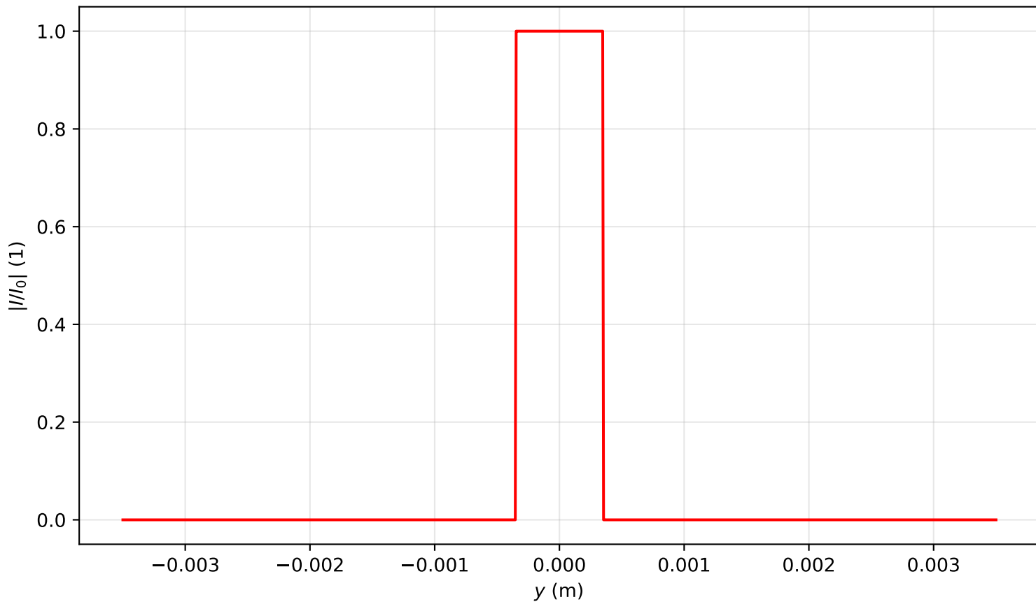
Intensity profile I(x = 0, y, z = 0.000)/I_0 , P_{in}=9.0P_{cr} , artificial time
